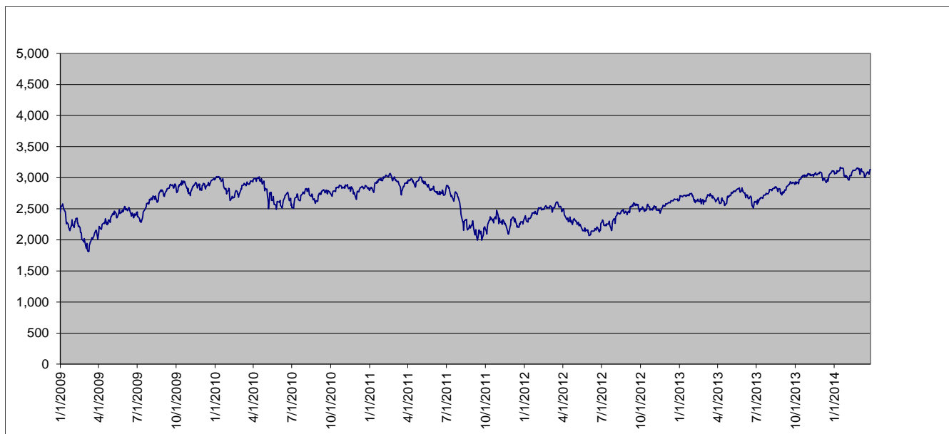
EURO STOXX 50® Index Daily Index Closing Values January 1, 2009 to March 27, 2014
